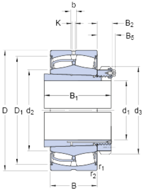
23052-2CS5K/VT143 + OH 3052 HE Bearing 2D drawings and 3D CAD models
