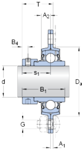
PF 40 WF Bearing 2D drawings and 3D CAD models
